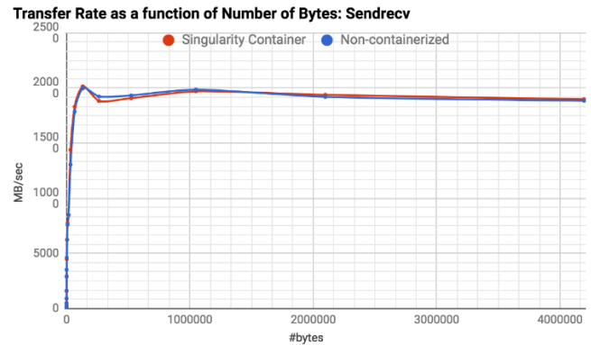
Figure 1: IMB Sendrecv Run using Singularity and Non-Singularity
